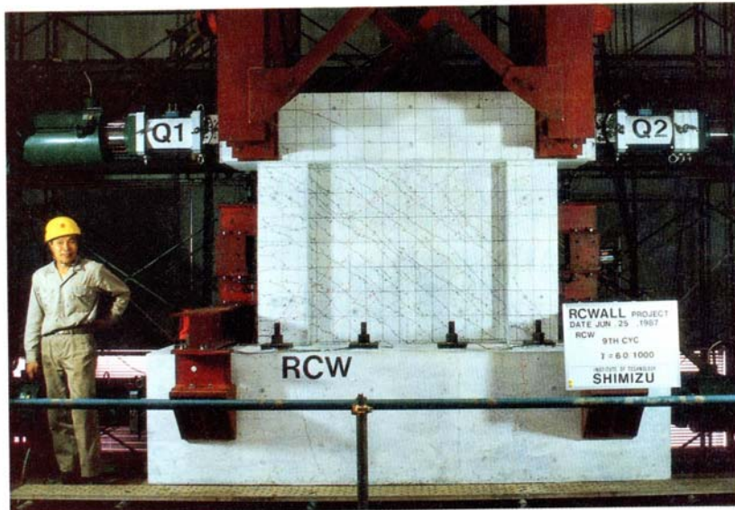
Reinforced concrete shear wall specimen
